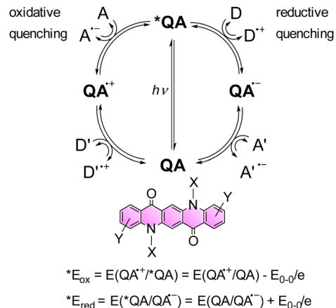
Scheme 3 Representation of possible reaction pathways of the *QA excited state through oxidative and reductive quenching, leading to the generation of oxidised QA + and reduced QA - , respectively. A and A' represent electron acceptors, while D and D' represent electron donors. The two equations enable the estimation of E_{ox} and E_{red} of the *QA excited state. 41,42
