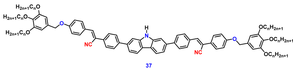
Fig. 25 Structure of compound 37 .
