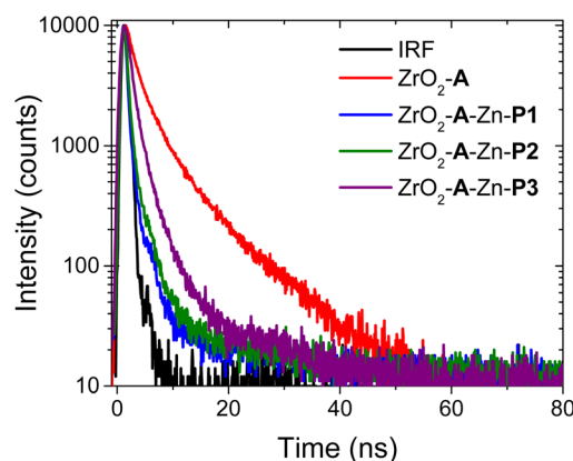
Fig. 3 Time-resolved emission at 460 nm for ZrO 2 - A and ZrO 2 - A -Zn- PX in MeCN ( \lambda_{\text{ex}} = 360 nm).
