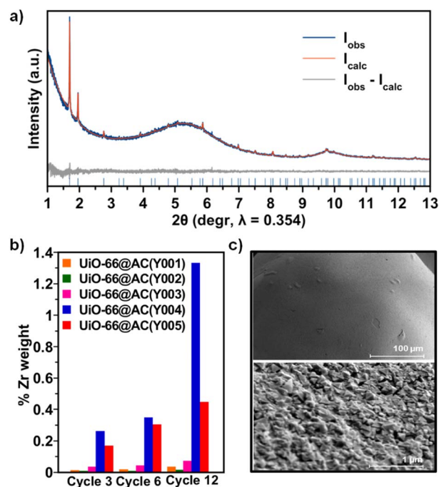
Fig. 2 (a) Graphical result of the whole powder pattern refinement carried out with the Le Bail method ( R_p = 0.022 ; R_{\text{wp}} = 0.019 ) on the HR-PXRD of as-synthesized UiO-66@AC(Y004) _{\text{HNO}_3} in terms of observed, calculated and difference traces (blue, red and grey, respectively). The positions of the Bragg reflection are indicated by blue ticks. Cell parameters: a = b = c 20.8288 (3) \text{\AA} , V = 9036.4 (3) \text{\AA}^3 ; (b) inductively coupled plasma analysis of Zr percentage in UiO-66@AC(Y00 n ) _{\text{HNO}_3} ( n = 1 –5) composites throughout different synthetic cycles; (c) SEM images of UiO-66@AC(Y004) _{\text{HNO}_3} .
