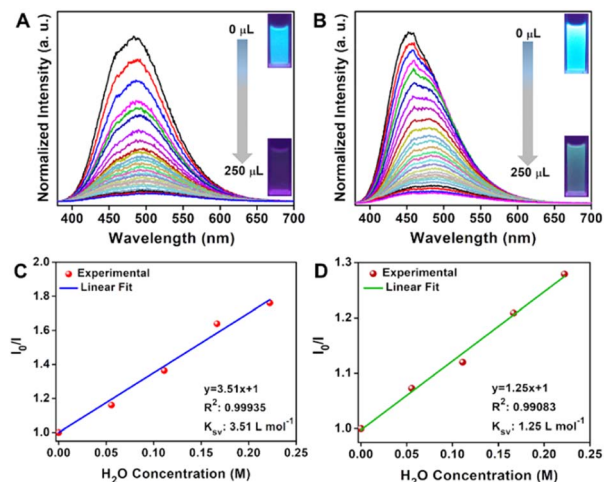
Fig. 5 (A) PL spectra of 1 dispersed in ACN showing the quenching of photoluminescence upon gradual addition of water (B) PL spectra of 1 dispersed in acetone showing the quenching of photoluminescence upon gradual addition of water (C) A Stern–Volmer plot at a low water concentration in ACN showing the linearity. (D) A Stern–Volmer plot at a low water concentration in acetone showing the linearity.
