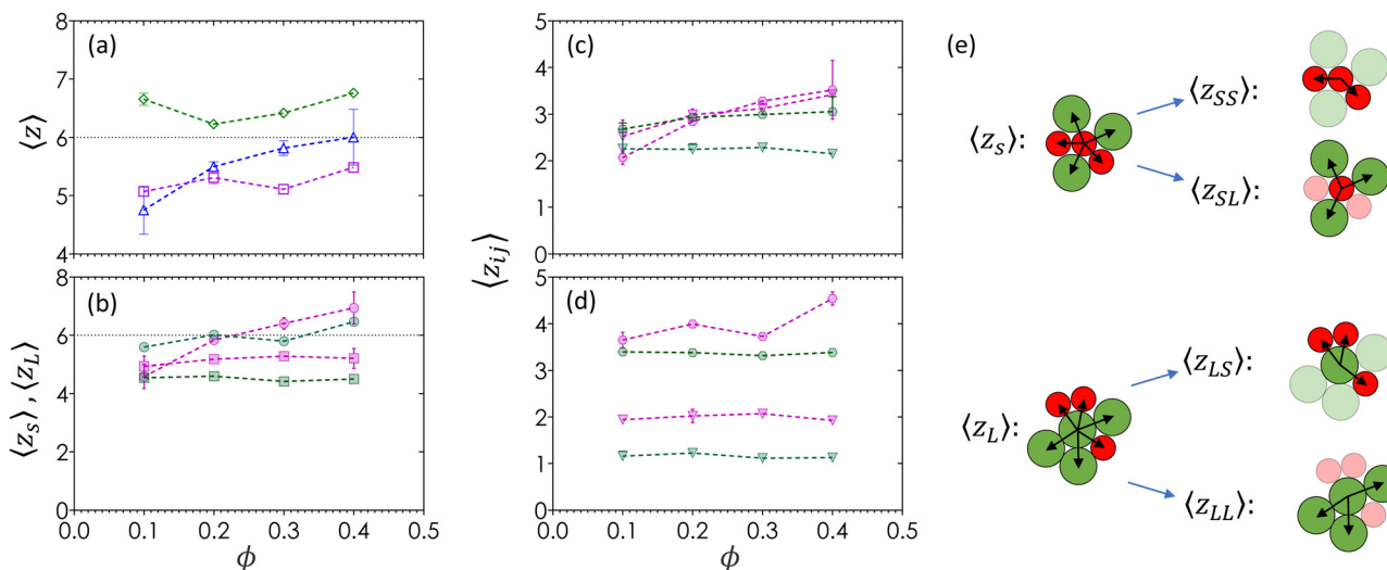
Fig. 5 (a) The average contact number \langle z \rangle plotted against \phi for monodisperse ( \alpha = 1.0 , green diamonds) and bidisperse systems ( \alpha = 0.72 , blue triangles; and \alpha = 0.60 , magenta squares). Dotted line at \langle z \rangle = 6 is equivalent to Maxwell's isostatic criterion. (b) Average contact number of small (green squares) and large particles (green circles) at \alpha = 0.60 , plotted alongside small (magenta squares) and large particles (magenta circles) at \alpha = 0.72 . Pairing specific contact number as a function of \phi for (c) \alpha = 0.72 and (d) \alpha = 0.60 , categorized by their pairing: SS (green triangles), SL (green hexagons), LS (magenta triangles), and LL (magenta hexagons). (e) Schematic that shows how pairing-specific contacts are categorized.
