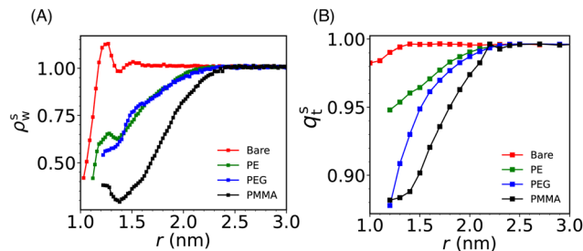
Fig. 3 (A) The scaled water density ( \rho_{\text{w}}^{\text{s}} ) profile in the radially outward direction from the center-of-mass of the Si-NP. (B) The same is shown for the scaled tetrahedral order parameter ( q_{\text{t}}^{\text{s}} ) of water. We note an enhanced density and tetrahedral order of water molecules around bare Si-NP and significantly lower water density and structural order in the vicinity of the PMMA-grafted Si-NP. We also note that, both the water density and structural (tetrahedral) order reach their respective bulk value at \sim 2.4 \text{ nm} from the center of the Si-NP for all the Si-NPs.
