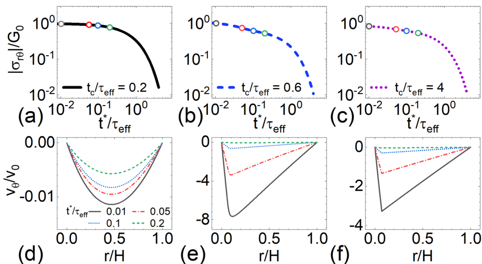
Fig. 9 Evolution of shear stress (a)–(c) and retraction velocity profiles (d)–(f) in cessation of flow following shear startup using the GCB model at Wi = 5 , for three stop times: t_c/\tau_{\text{eff}} = (a) and (d) 0.2, (b) and (e) 0.6, and (c) and (f) 4. Shear stress at the inner cylinder ( r/H = 0 ) is normalized by the elastic modulus at rest, G_0 . Velocity is normalized by the imposed wall velocity v_0 ; velocity profiles are shown at four times, t^*/\tau_{\text{eff}} , during the stress relaxation following flow cessation (denoted by \circ in a–c).
