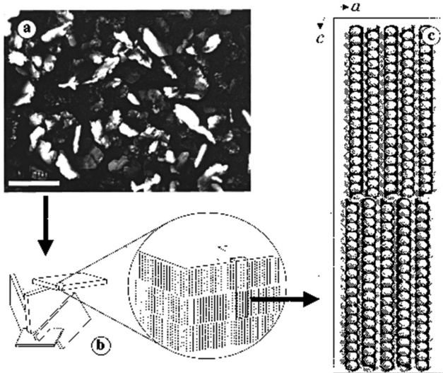
Fig. 5 (a) Optical micrograph of a 4 wt% C_{36}H_{74}/1 -octanol gel viewed through crossed polars (scale bar = 100 \mu\text{m} ), (b) a cartoon representation of the micro-platelets showing the orientations of the long molecular axes of C_{36}H_{74} molecules, and (c) the molecular packing of C_{36}H_{74} . Figure reproduced from ref. 56 with permission from the American Chemical Society, © 2000.
