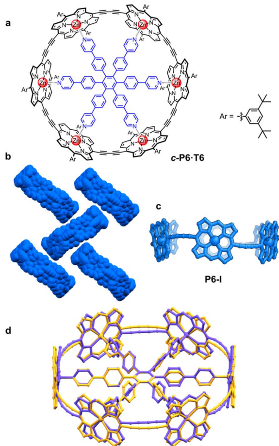
Fig. 1 (a) Drawing of a six-porphyrin nanoring with the template marked in blue, Ar = 3,5-di- tert -butylphenyl. (b) Fragment of the crystal structure of the previously reported, orthorhombic ( Pncc ) polymorph P6-I (CCDC: 860774). 6 (c) View of the molecular conformation of the nanoring in P6-I . Hydrogen atoms, template and aryl groups in (b) and (c) are omitted for clarity. (d) Comparison of the molecular geometry of c-P6·T6 from the published crystal structure of polymorph P6-I (purple) 6 and the gas-phase geometry from DFT calculations (BLYP35/6-31G*, yellow). 16
