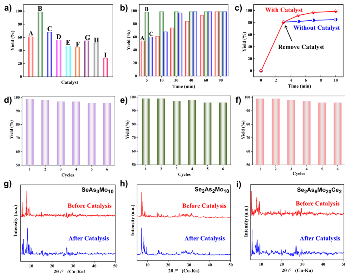
Fig. 4 (a) Catalytic efficiency of the different catalysts in the model reaction ((A) SeAs 3 Mo 10 ; (B) Se 2 As 2 Mo 10 ; (C) Se 2 As 6 Mo 20 Ce 2 ; (D) As 4 Mo 12 ; (E) (NH 4 ) 6 Mo 7 O 24 ·4H 2 O; (F) p -H 2 NC 6 H 4 AsO 3 H 2 ; (G) SeO 2 ; (H) mixture; (I) no catalyst). (b) Catalytic efficiency of SeAs 3 Mo 10 (A), Se 2 As 2 Mo 10 (B), and Se 2 As 6 Mo 20 Ce 2 (C) as a function of time. (c) Results of the filtration test conducted on the Se 2 As 2 Mo 10 heterogeneous catalyst. (d)–(f) Catalytic stability of SeAs 3 Mo 10 (d), Se 2 As 2 Mo 10 (e), and Se 2 As 6 Mo 20 Ce 2 (f) (error bar \pm 1\% ). (g)–(i) Powder XRD patterns of SeAs 3 Mo 10 , Se 2 As 2 Mo 10 , and Se 2 As 6 Mo 20 Ce 2 before and after catalysis.
