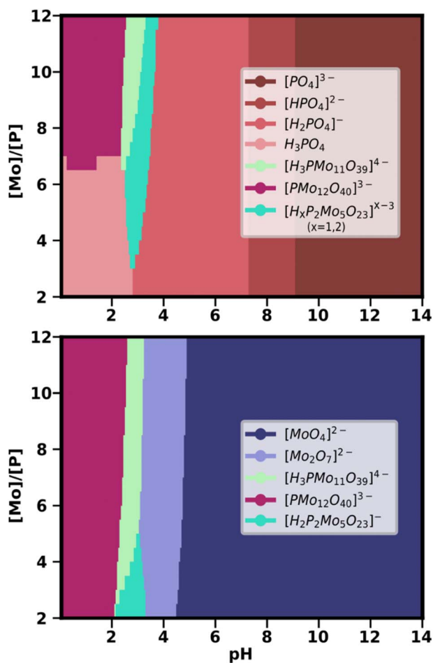
Fig. 5 Speciation phase diagram for the PMo system. The horizontal axis represents pH and the Y axis represents the [Mo]/[P] ratio. The top diagram shows as phosphorus percentage and the bottom one as the molybdenum percentage. The diagrams correspond to two different views of the same speciation phase diagram.
