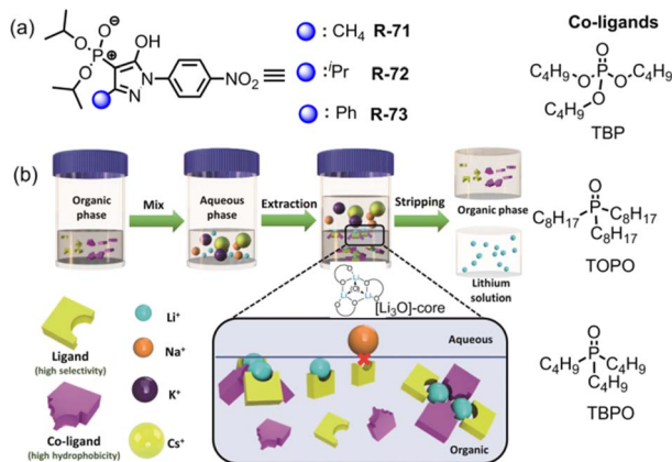
Fig. 21 (a) Chemical structure of the receptors R-71 to R-73. (b) Schematic illustration of the Li + extraction process with the presence of receptor and co-ligand. Reproduced with permission from ref. 105. Copyright 2022, Chemistry – A European Journal published by Wiley-VCH GmbH.
