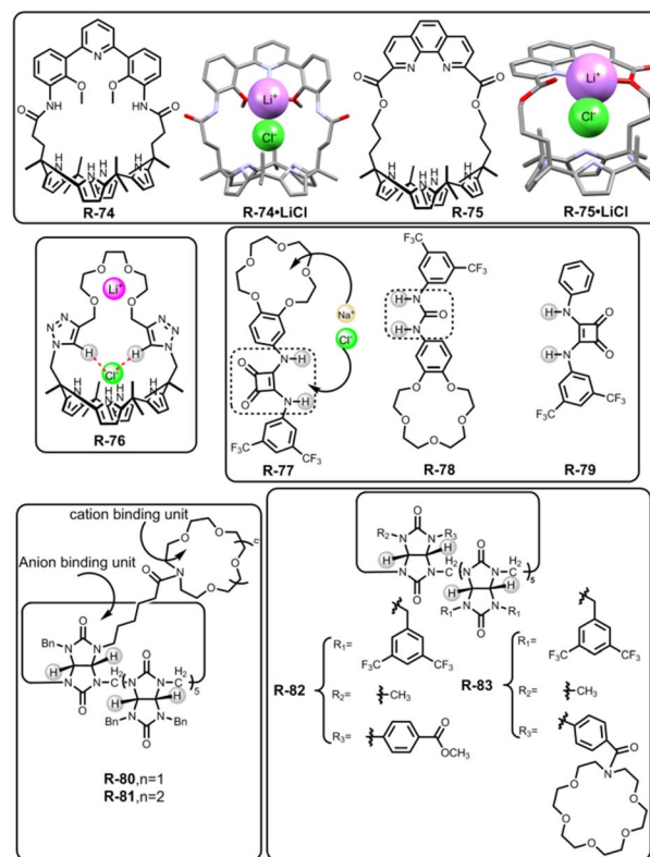
Fig. 23 Chemical structure of the receptors R-74 to R-83 and crystal structures of R-74-LiCl and R-75-LiCl (data from the Cambridge Crystallographic Data Centre [CCDC # 1821811 and 1821810 respectively]). 110
