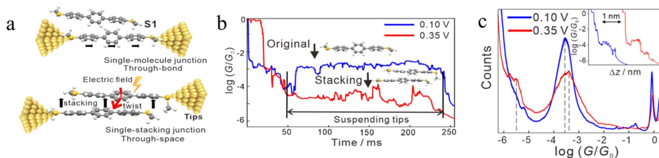
Fig. 19 (a) Schematic of single-molecule junctions and single-stacking junctions of a SMe anchored terphenyl derivative; (b) two typical traces with the suspended retracting process under 0.10 (blue) and 0.35 V (red) for terphenyl; (c) 1D conductance histograms and typical conductance–displacement traces (inset) under 0.10 (blue) and 0.35 V (red); the black dashed line indicates the position of the conductance peak, and the inset shows typical traces. Figures adapted with permission from ref. 92. Copyright 2020, American Chemical Society.
