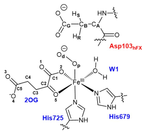
Fig. 2 QM region used for the QM/MM calculations of the AspH reaction mechanism includes Fe, 2OG (superoxo), O 2 (superoxo), succinate (ferryl), oxo (ferryl), side chain imidazole rings of Fe-ligating histidines (His679 and His725), W1 (mode A), Asp103 hFX .
