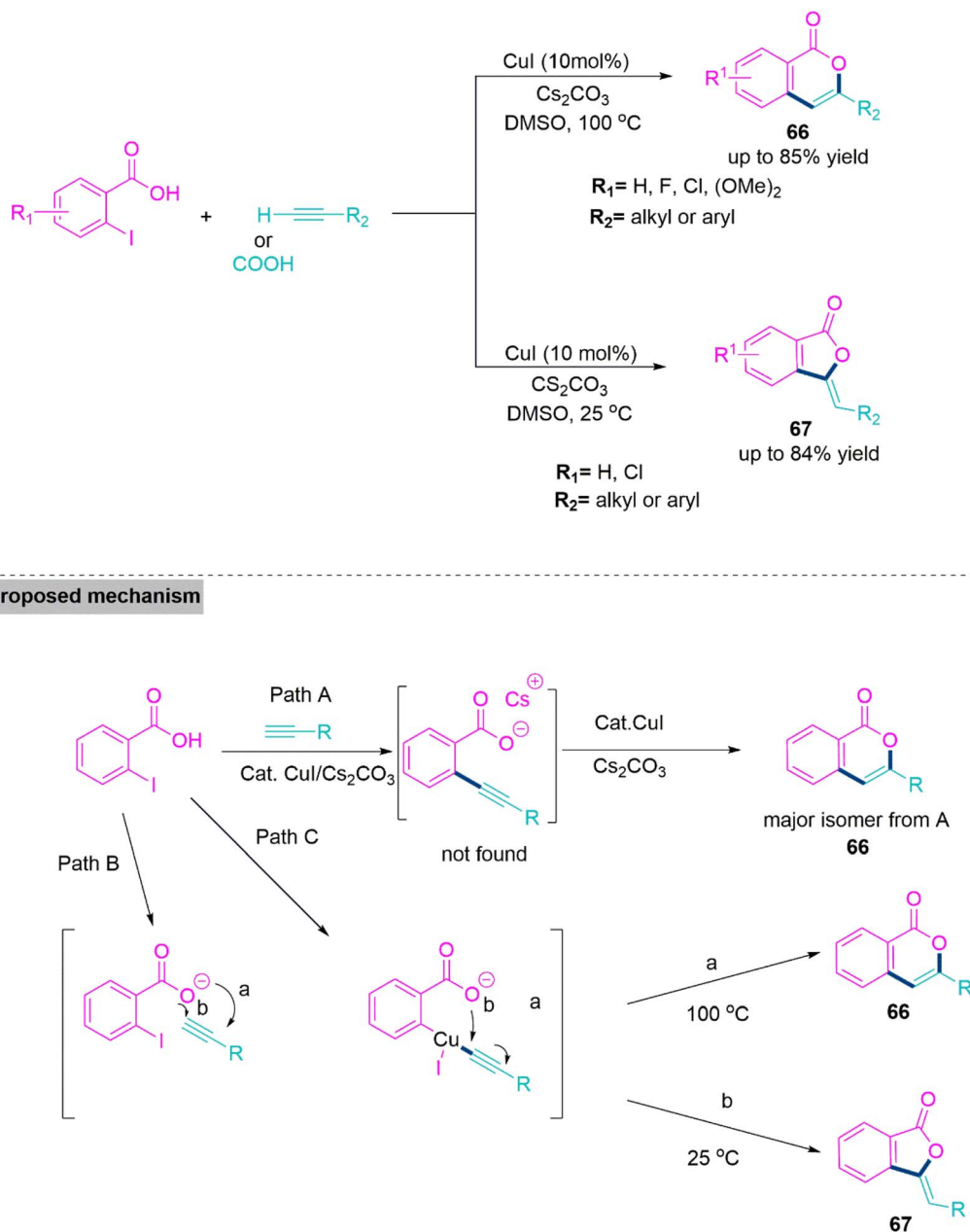
Scheme 35 Synthesis of isocoumarins (66) and phthalide derivatives (67).
