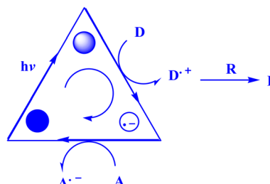
Fig. 5 Reductive quenching-oxidative activation. 174
