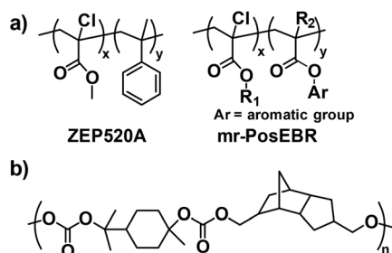
Fig. 13 Non-chemically amplified resists based on main-chain scission. (a) PMMA derivatives ZEP520A and mr-PosEBR. (b) Polycarbonate polymers with EUV-sensitive carbonate moieties and alicyclic groups.
