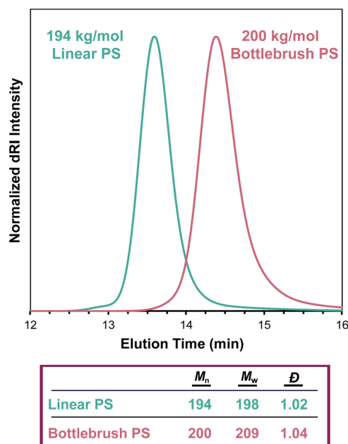
Fig. 8 SEC-MALS chromatograms of a 194 \text{ kg mol}^{-1} linear PS sample (teal trace, nominal 200 \text{ kg mol}^{-1} standard) and a 200 \text{ kg mol}^{-1} bottlebrush PS sample (pink trace), showing the difference in elution time as a result of polymer topology.
