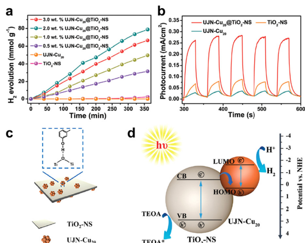
Fig. 9 (a) Photocatalytic H 2 production rates of composite catalysts with different UJN-Cu 20 cluster loadings using a 300 W xenon lamp as the light source to simulate sunlight. (b) Photo-response current density of UJN-Cu 20 , TiO 2 -NS and UJN-Cu 20 /TiO 2 -NS. (c) Schematic diagram of the interaction of UJN-Cu 20 with TiO 2 -NS surface. (d) Schematic illustration of the relative positions of the UJN-Cu 20 and TiO 2 -NS energy bands and the electron transfer mechanism over the composite catalysts. Reproduced with permission from ref. 77. Copyright 2021 Royal Society of Chemistry.
