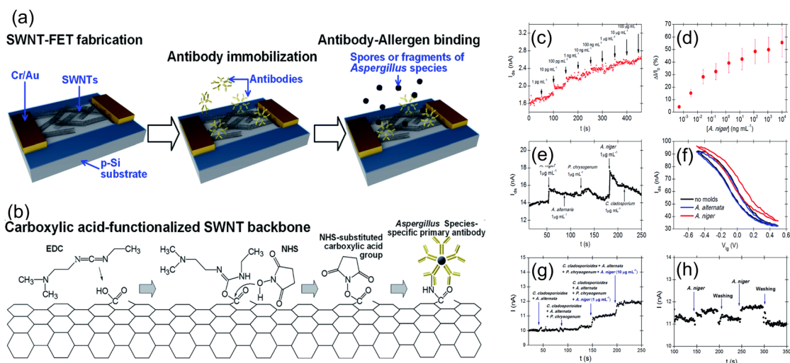
Fig. 13 (a) Illustration of the antibody–allergen binding and the fabrication of fungi sensors based on SWNT-FETs for binding of allergens. (b) EDC/NHS chemistry was utilized to immobilize WF-AF-1 Abs directly onto the carboxylic acid-functionalized SWNT surface. (c) The real-time response of an SWNT-FET device immobilized with WF-AF-1 Abs to a series of injections of varying concentrations of A. niger -suspended PBS solution. (d) Corresponding calibration curve. (e) Response of the functionalized SWNT-FET device in real-time to a random succession of administrations of various mould-suspended PBS solutions. (f) Sensor possesses a liquid gating effect that is specific to target and non-target molds. (g) Injection of four distinct mixtures of fungal solutions sequentially. The initial two mixtures do not contain A. niger , whereas the final two mixtures do contain A. niger in ten-fold different concentrations. (h) Water and PBS buffer are used to thoroughly rinse the sensor to revive it. Reprinted with permission from ref. 39 (copyright © 2015 Published by RSC advance).
