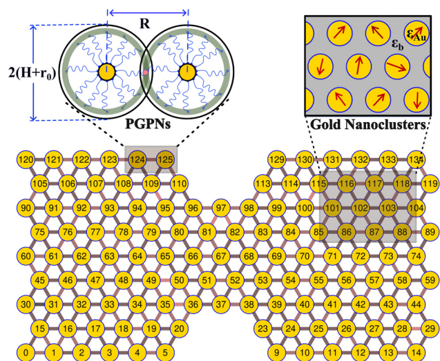
Fig. 1 The PGPNSs are composed of gold nanoparticle cores with radius r_0 = 25 nm and f = 900 polymers grafted on their surface. The pair interactions between the PGPNSs help them to form a stable cross-linked network. Equilibrated double notched PGPNSs arranged in a hexagonal lattice are stable and form gold nanoclusters with dipole moments that depend on the interaction between the PGPNSs that form the array.
