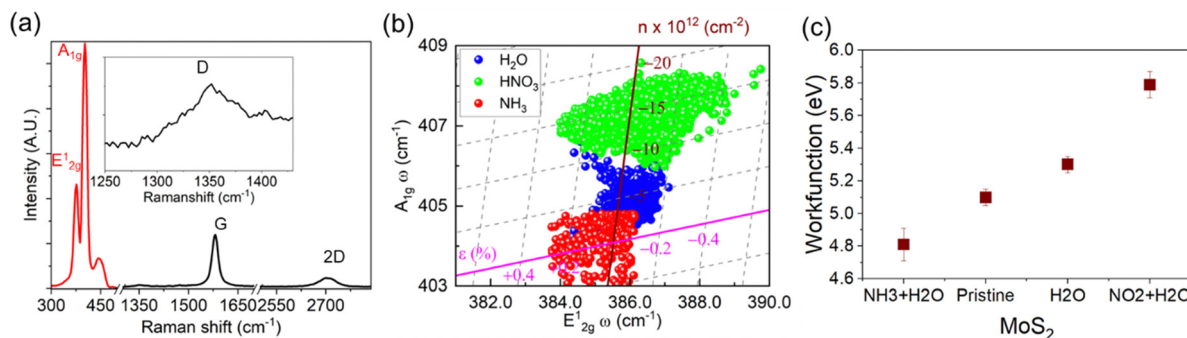
Fig. 3 Analytes induced doping in MoS 2 . (a) Raman spectrum of the hybrid structure showing Raman modes of MoS 2 (E 2g 1 and A 1g ) and few-layer graphene (G and 2D). (b) Correlation plot (E 2g 1 vs. A 1g ) shows the shift in peak position in the MoS 2 Raman modes after exposure of solvents of dilute HNO 3 (as NO 2 + H 2 O), NH 4 OH (as NH 3 + H 2 O) and H 2 O. (c) Trend of work function (eV) of MoS 2 in different exposures of analytes.
