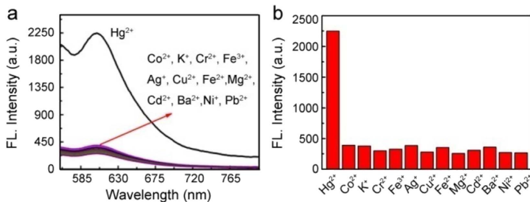
Fig. 4 (a) Fluorescence spectra for the fluorophore-labeled \text{Au@SiO}_2 probe in the presence of 1.0 equivalent of \text{Hg}^{2+} , \text{Co}^{2+} , \text{Fe}^{3+} , \text{Cd}^{2+} , \text{Fe}^{2+} , \text{K}^+ , \text{Cr}^{2+} , \text{Cu}^{2+} , \text{Pb}^{2+} , \text{Mg}^{2+} , \text{Ag}^+ , \text{Ba}^{2+} , and \text{Ni}^{2+} . The final concentration of the probe and metal ions are all 0.5 \mu\text{M} . (b) Selectivity of NP sensors plotted in histogram form.
