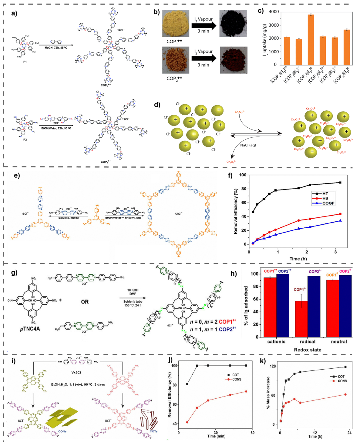
Fig. 5 (a) Synthesis of COP 1 + and COP 2 + . (b) Real images of iodine vapor adsorption in COP 1 and COP 2 at 60 °C. (c) Iodine vapor capture capacities of COP 1 and COP 2 in three different redox states. (d) Schematic representation of anion removal (MnO 4 - , Cr 2 O 7 2- ) by anion exchange, where yellow spheres represent polymer particles (COP 1 and COP 2 ). Reproduced with permission from ref. 70. Copyright 2014 the Royal Society of Chemistry. (e) Synthesis of the hollow sphere (HS) and hollow tube (HT) via the solvothermal synthesis approach and the covalent organic gel framework (COGF) via the microwave synthesis approach. (f) Graph of % removal of I 2 from a 1 mM solution in cyclohexane over time by HT, HS and COGF. Reproduced with permission from ref. 43. Copyright 2022, American Chemical Society. (g) Synthesis of COP 1 + and COP 2 + . (h) Solution-phase iodine adsorption by the three redox states of COP 1 and COP 2 . Reproduced with permission from ref. 69. Copyright 2022 Wiley-VCH. (i) Synthesis of CONs and COTs, (j) and (k) iodine adsorption experiments. Reproduced with permission from ref. 89. Copyright 2022 Wiley-VCH.
