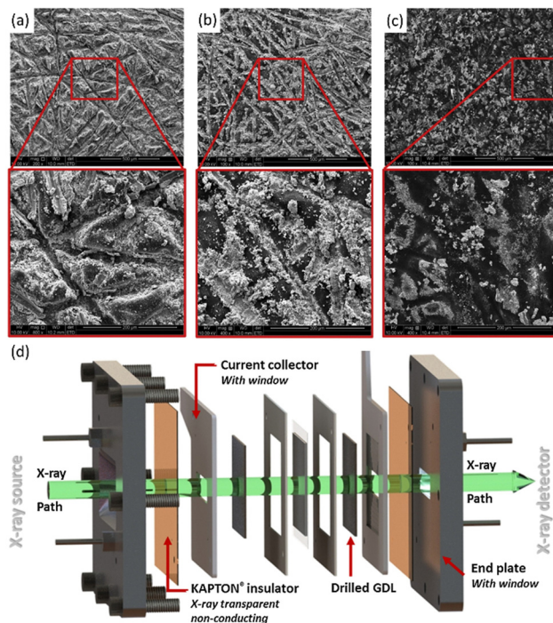
Fig. 7 Top-down SEM images of \text{NiFe}_2\text{O}_4 anode catalyst layers on (a) Sustainion, (b) Aemion, and (c) Tokuyama A201 membranes at (top) 100 \times and (bottom) 400 \times magnification. Reprinted from Pushkareva et al. , Comparative Study of Anion Exchange Membranes for Low-Cost Water Electrolysis, Int. J. Hydrog. Energy , 45 (49), 26070–26079, Copyright (2020), with permission from Elsevier. 179 (d) Schematic of PEMWE cell developed for in situ XAS measurements. Reprinted from Ampurdanés et al. , Cobalt-Based Oxide Materials as Non-PGM Catalyst for HER in PEM Electrolysis and In situ XAS Characterization of Its Functional State, Catal. Today , 336 , 161–168, Copyright (2019), with Permission from Elsevier. 193
