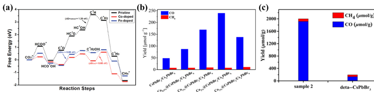
Fig. 10 (a) The free energy diagrams of the most favored paths of CO 2 reduction in pristine, Co-doped and Fe-doped cases. The DG ‡ of the rate-determining step for each case is listed. 105 (b) The yields of CO and CH 4 generated from photocatalytic CO 2 reduction in pure water based on undoped and Co-doped CsPbBr 3 /Cs 4 PbBr 6 with various doping concentrations. 55 (c) Comparison chart of the yields between Mn-doped optimum catalyst sample 2 and CsPbBr 3 . 106
