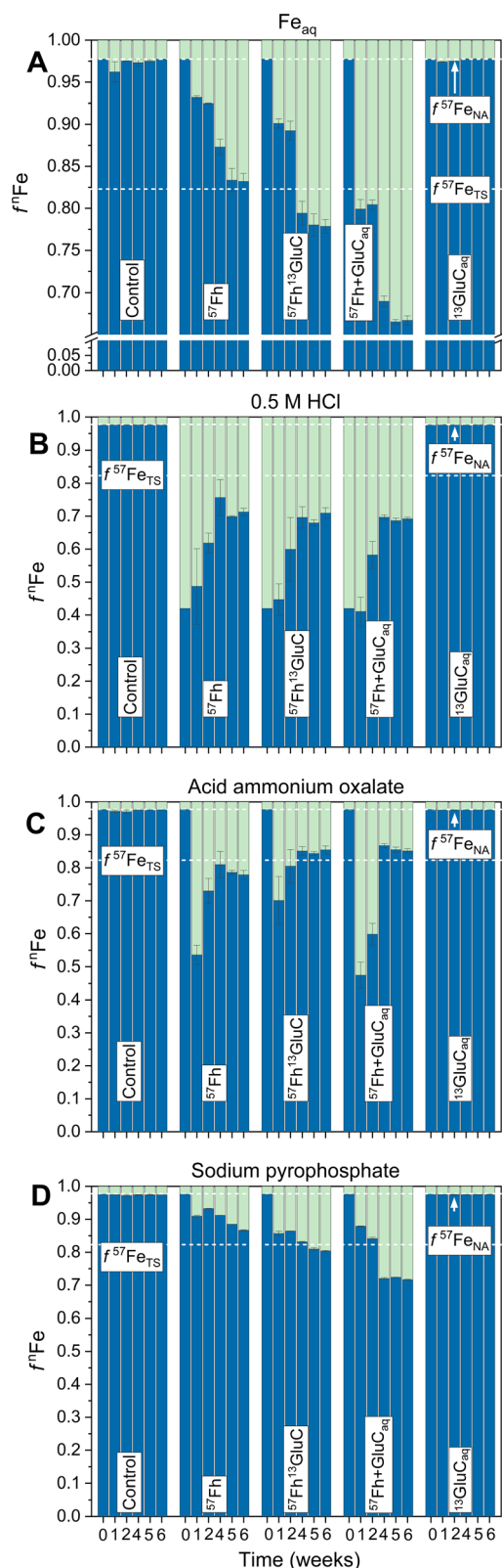
Fig. 1 Trends in Fe isotope composition of \text{Fe}_{\text{aq}} (A) and the selective chemical extractions, shown as f^{n}\text{Fe} , where n = 56 (blue) or 57 (green). (B) and (C) are steps 1 and 2 of the two-step sequential extraction whereby (B) is total Fe extracted with 0.5 M HCl (2 h) and (C) is Fe mobilized with an acid ammonium oxalate extraction. Panel (D) shows the isotope composition of Fe mobilized in the Na-pyrophosphate treatment. The initial timepoint (week 0) is calculated based on the
