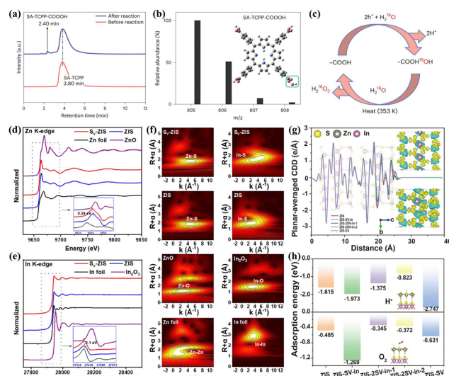
Fig. 6 (a) HPLC for SA-TCPP before and after reaction. 84 (b) The molecular ion peak obtained from the ESI(–)-TOF-MS spectrum for the 2.4 min HPLC peak. Inset is the molecular structure of SA-TCPP-COOOH. 84 (c) The mechanism for H 2 O 2 production on SA-TCPP by holes according to the isotopic experiments. 84 Normalized XANES spectra of S v -ZIS and ZIS at (d) the Zn K-edge and (e) the In K-edge. The inset is the first derivative of XANES spectra. 86 (f) Wavelet transform analysis of the k 3 -weighted EXAFS for S v -ZIS and ZIS at the Zn K-edge and the In K-edge. 86 (g) Planar-averaged CDD of ZIS, ZIS-S v -In, ZIS-2S v -In, ZIS-2S v -In-2, and ZIS-S v . 86 (h) Adsorption energy of H + and O 2 on the S site of the different models. 86
