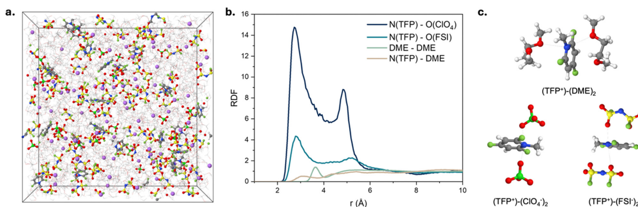
Fig. 4 (a) A snapshot of the MD simulation cell for 0.91 M LiFSI and 0.27 M [TFP][ClO 4 ] in DME. (b) Radial distribution functions for 0.91 M LiFSI and 0.27 M [TFP][ClO 4 - ] in DME at 298 K and (c) representative cation solvates for 0.91 M LiFSI and 0.27 M [TFP + ][ClO 4 - ] in DME at 298 K.
