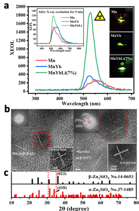
Fig. 19 (a) X-ray excited luminescence spectrum and afterglow spectrum (inlet) of Mn, MnYb, and MnYbLi (7%) samples after X-ray excitation for 5 min. (b) High resolution TEM images of \text{Zn}_2\text{SiO}_4:\text{Mn} ( \alpha/\beta = 0.42 , left) and \text{Zn}_2\text{SiO}_4:\text{Mn,Yb,Li} ( \alpha/\beta = 3.57 , right) samples. (c) XRD patterns of \alpha - \text{Zn}_2\text{SiO}_4 and \beta - \text{Zn}_2\text{SiO}_4 . Reproduced with permission from ref. 210. Copyright 2023, American Chemical Society.
