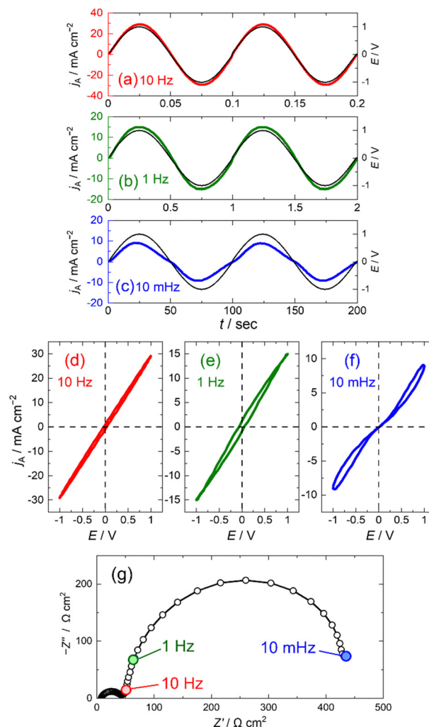
Fig. 2 (a)–(c) Applied voltage and output current for polarisation measurements; (d)–(f) steady-state polarisation curves of a LAMO/LAMO symmetric cell at -15^{\circ}\text{C} . The frequency of applied voltage was (a) and (d) 10 Hz, (b) and (e) 1 Hz and (c) and (f) 10 mHz. (g) The Nyquist plot of the LAMO/LAMO symmetric cell measured at -15^{\circ}\text{C} .
