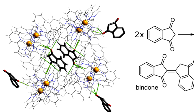
Fig. 8 Cage-catalysed aldol condensation of indane-1,3-dione to binone; the crystal structures show both cavity binding of neutral indane-1,3-dione guests (stacked pair across an inversion centre) plus external surface-binding of additional units presumed to be enolate anions, illustrating the ability of the cage to co-locate cavity-based (neutral) and surface-based (anionic) guests.
