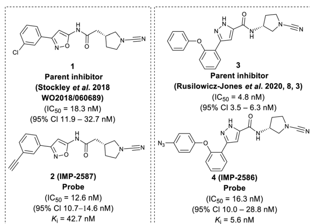
Fig. 1 Chemical structure of parent compounds and activity-based probes with their determined IC 50 and K_i accordingly. Fluorescent Polarisation assay were performed for IC 50 (30 minutes incubation against USP30), k_{\text{obs}}/I , and k_{\text{inact}}/K_i determination of IMP-2587 , and IMP-2586 against USP30 using Ub-Lys(TAMRA)-Gly (Fig. S1, ESI†).
