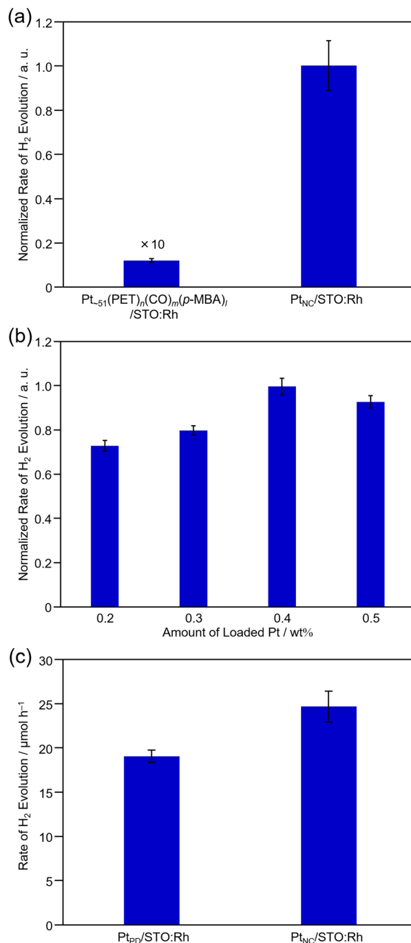
Fig. 5 \text{H}_2 -evolution activity of Pt cocatalyst-loaded STO:Rh photocatalysts. (a) Before ( \text{Pt}_{51}(\text{PET})_n(\text{CO})_m(p\text{-MBA})_l/\text{STO:Rh} ) and after ( \text{Pt}_{\text{NC}}/\text{STO:Rh} ) calcination of Pt NC-loaded STO:Rh and (b) dependence of loading weight of the Pt cocatalyst for \text{Pt}_{\text{NC}}/\text{STO:Rh} . (c) Comparison of \text{H}_2 -evolution activity between \text{Pt}_{\text{NC}}/\text{STO:Rh} and \text{Pt}_{\text{PD}}/\text{STO:Rh} . In (a) and (c), the loading weight of Pt on them was 0.4 wt%. In order to eliminate the effect of the difference in the activity of each photocatalyst, STO:Rh synthesized in the same batch was used in each experiment (a)–(c).
