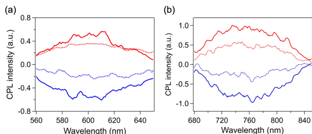
Fig. 6 CPL spectra of (a) IrAu 12 -R (red) and IrAu 12 -S (blue) in MeTHF and (b) Au 13 -R (red) and Au 13 -S (blue) in a MeOH–EtOH mixture (1:1 v/v) recorded at the excitation wavelength of 375 nm. Solid and dotted lines denote the spectra recorded at 200 and 300 K, respectively.
