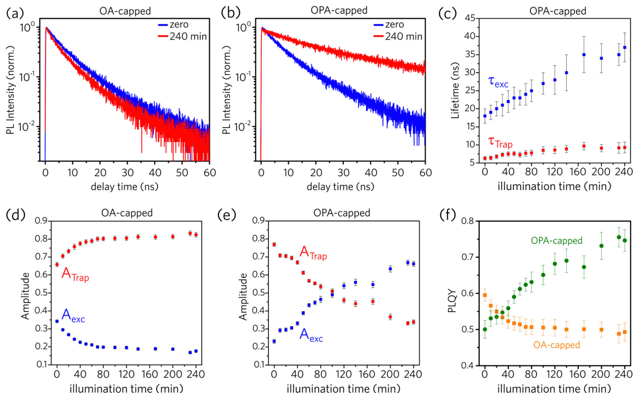
Fig. 5 PL dynamics as a function of illumination time for (a) OA-capped and (b) OPA-capped CsPbBr 3 PNCs. (c) Calculated lifetimes ( \tau ) from PL decay data for OPA-capped PNCs. Calculated amplitudes ( A ) from PL decay data for (d) OA-capped and (e) OPA-capped PNCs ( A_{\text{Trap}} : trap-assisted recombination; A_{\text{exc}} : excitonic recombination). (f) Calculated photoluminescence quantum yield (PLQY) from PL decay data for OA- and OPA-capped PNCs.
