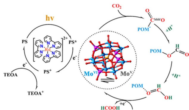
Scheme 7 Proposed mechanism for the photocatalytic \text{CO}_2 reduction to \text{HCO}_2\text{H} catalyzed by NU-29. Reprinted from ref. 88 with permission from American Chemical Society (Copyright 2019).
