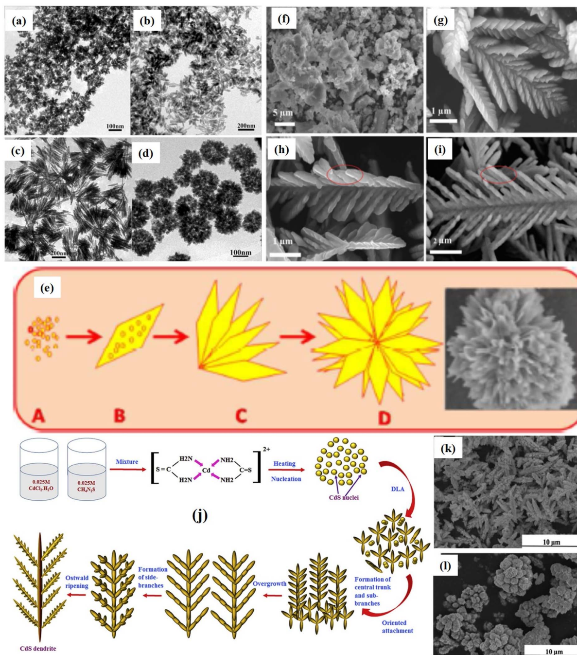
Fig. 6 (a–d) 3D CdS hierarchical nanostructures i.e. water lily, nanorices, nanofans and porous microparticles under different experimental conditions. Schematic representation of the formation of CdS dendrites. Reprinted with permission from ref. 112. (e) Schematic of mechanism of growth of 3D CdS hierarchical nanoflower. Reprinted with permission from ref. 113. Formation of CdS dendrites nanostructures: SEM images of samples prepared at different temperatures: (f) 120, (g) 150, (h) 180, and (i) 220 °C. Reprinted with permission from ref. 114. (j) Schematic of mechanism for the growth of hierarchical CdS dendrites 115 (k and l) Zn-doped dendritic-like CdS structures (k) Zn-doped lower concentration and (l) higher concentration. Reprinted with permission from ref. 116.
