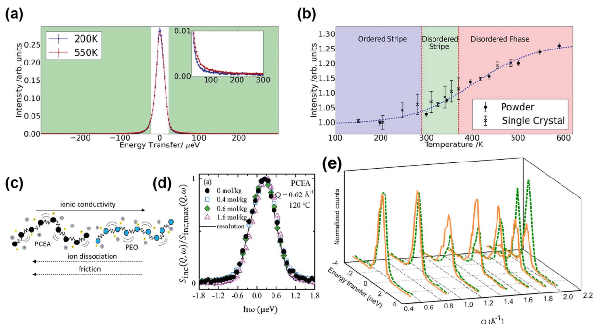
Fig. 23 (a) QENS spectra from \text{Na}_{0.8}\text{CoO}_2 at T \approx 200 K (blue) and T \approx 550 K (red) integrated over Q . Inset shows increase in the quasi-elastic region. (b) QENS intensity integrated over Q and energy transfer as a function of temperature for the powder and single-crystal samples of \text{Na}_{0.8}\text{CoO}_2 . 101 Copyright 2018, CC BY 4.0. (c) Representation of PEO and PCEA polymers. (d) Normalized incoherent structure factor, S_{\text{inc}}(Q, \omega)/S_{\text{inc}, \text{max}}(Q, \omega) , in the frequency domain, plotted as a function of energy, \hbar\omega , at Q = 0.62 \text{ \AA}^{-1} and 120 C. Reprinted with permission from ref. 103 Copyright (2020) American Chemical Society. (e) QENS spectra recorded for {}^7\text{Li}(\text{BD}_4)_{0.75}\text{Li}_{0.25} , at 300 K, without (orange solid line) and with (green dashed line) the application of a potential ( f = 1 \text{ kHz} , U = 3 \text{ V} , and I = 0.4 \text{ mA} ). 107 Reprinted with permission from ref. 107 Copyright 2013 American Chemical Society.
