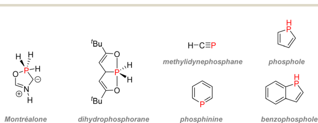
Fig. 10 Examples of phosphorus-containing heterocycles.
