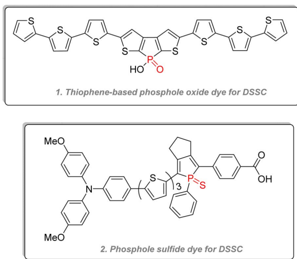
Fig. 28 Phospholes used for dye-sensitized solar cells.
