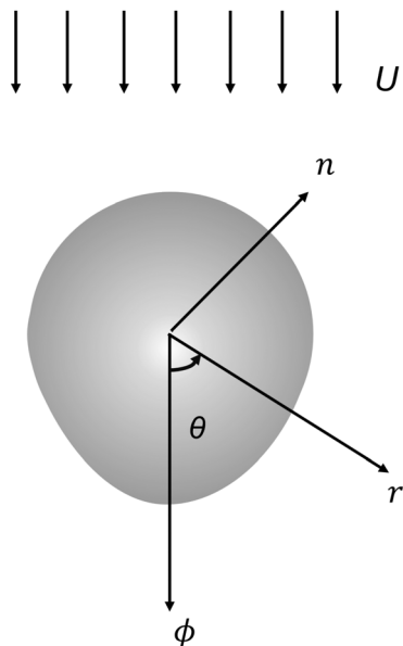
Fig. 5 Schematic of a deformed droplet as adapted from ref. 69.
