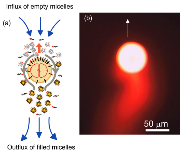
Fig. 1 (a) Schematic of micellar solubilization induced self-propulsion of droplets. (b) Fluorescence micrograph of an active 5CB droplet (50 \mu m) tagged with Nile red fluorescent dye releasing a trail of filled micelles.
