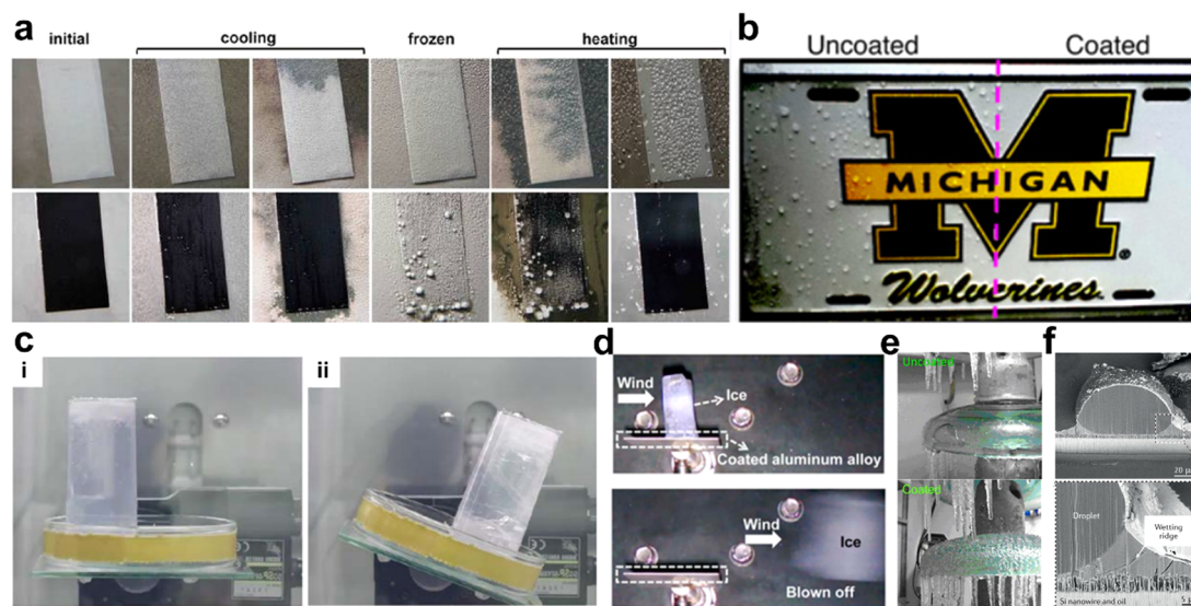
Fig. 13 Anti-icing with SLIPS. (a) The comparison of anti-icing performance between the original aluminum and the aluminum with a slippery coating. The records clearly showed that the slippery coating not only prevents the ice nucleation on the surface but also promotes the removal of melty ice. 48 (b) Half-coated license plate during outdoor winter 2013 testing, with ice only accreted on the uncoated side. 21 (c) Anti-icing properties of organogels prepared on Petri dishes (AR20 and TSF437 were mixed as organic phases). 123 (d) Effectiveness of the anti-icing coating with an aqueous lubricating layer was tested in the wind tunnel. The ice on the anti-icing could be blown off with a strong breeze. Arrows denote the direction of the wind. 122 (e) Ice formed on PDMS coated and uncoated surfaces of an insulator under a condensing weather condition at -5\text{ }^{\circ}\text{C} and saturated humidity. 120 (f) The cryogenic scanning electron microscope images revealed that the infused liquid may cloak the droplet during the icing formation, indicating a possible reason for the anti-icing property. 31
