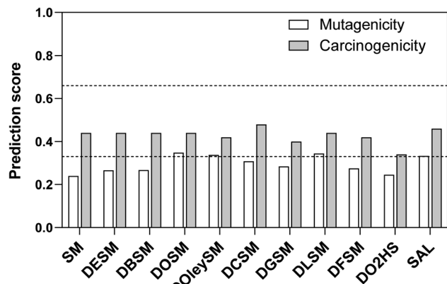
Fig. 7 Schematic presentation of the results of the in silico analysis with regard to the endpoint mutagenicity, and carcinogenicity. The test compounds are listed by their average prediction score on the y axis. In addition, the prediction scores were divided in three different groups (dashed lines): the probable mutagens/carcinogens with scores greater than 0.66, the probably non-mutagens/non-carcinogens with scores smaller than 0.33, and the remaining equivocal predictions with scores between 0.33 and 0.66.
