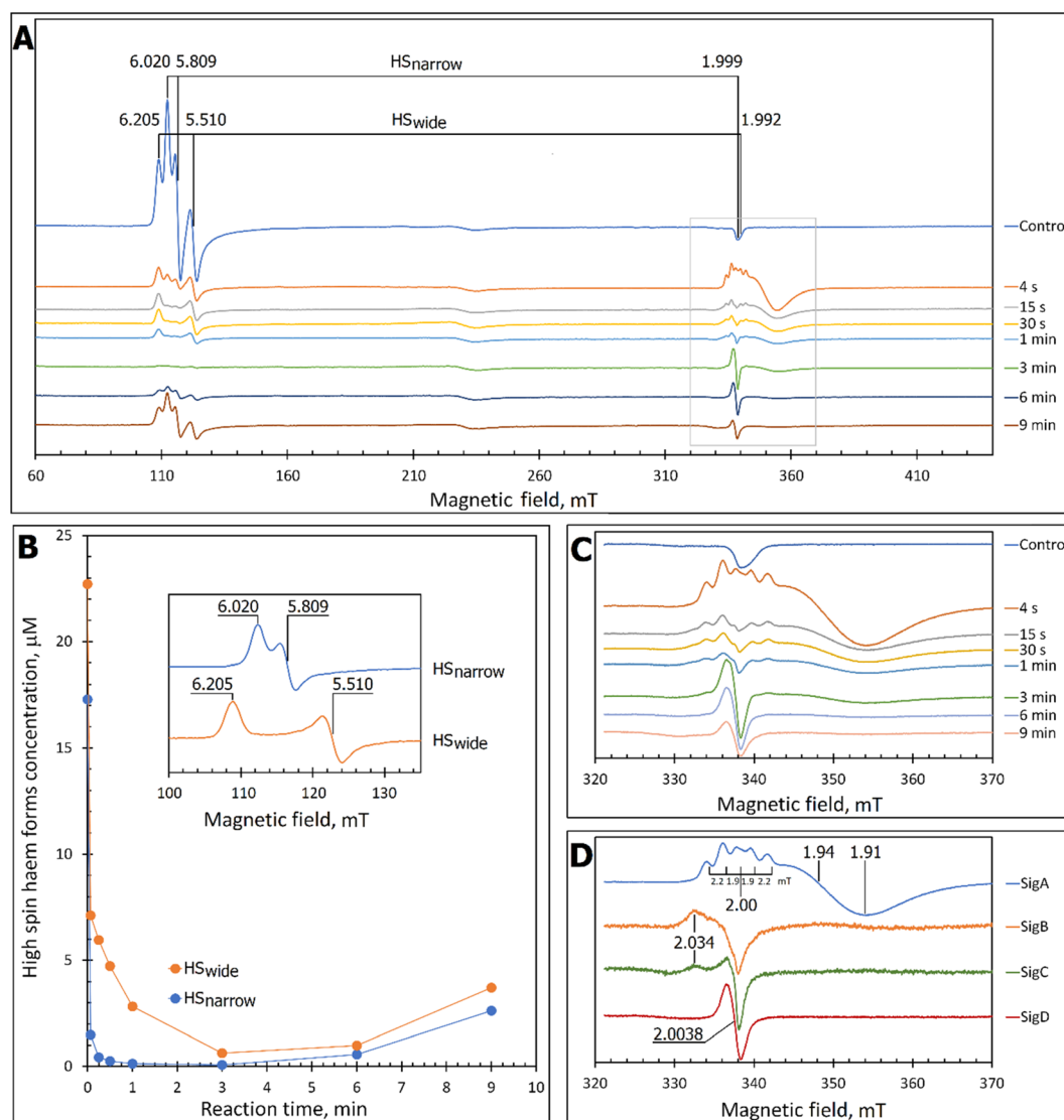
Fig. 2 X-band CW EPR spectroscopy of DtpAa upon reaction with H 2 O 2 at 10 K and pH 5.0. (A) The EPR spectra of DtpAa before (Control) and at different times after mixing with 400 \mu\text{M} H 2 O 2 . The g -values of the two HS ferric heme forms, HS narrow and HS wide , are indicated and are consistent with those previously reported. 36 The signal at \sim 230 millitesla is a background contribution. (B) The kinetic dependences averaged over two independent experiments of the two HS ferric heme forms. The inset gives the respective line shapes of the two HS signals, in the g = 6 region, extracted by spectral subtraction with variable coefficient, 48 formulated as follows: HS narrow = (Control) – 3.3 \times (4 s); HS wide = (4) – 0.084 \times (Control). (C) Detailed view of the spectral region covering the field interval of 320–370 mT within the grey frame in (A). All instrumental conditions used were the same as in (A) (see Experimental section) but with a slower R_S = 0.325 \text{ mT s}^{-1} . (D) The spectral components (pure line shapes) contributing to the EPR spectra shown in C. All signals (SigA to SigD) were obtained by using the procedure of spectra subtraction with variable coefficient, 48 formulated as follows; SigA = (4 s) – 0.23 \times (Control); SigB = (15 s) – 0.61 \times (4 s) – 0.145 \times (1 min); SigC = (1 min) – 0.61 \times (4 s) – 0.392 \times (15 s); SigD = (6 min) – 0.337 \times (3 min). The g -values of spectral points of interest are indicated and the distances between the hyperfine components of SigA, are indicated in millitesla.
