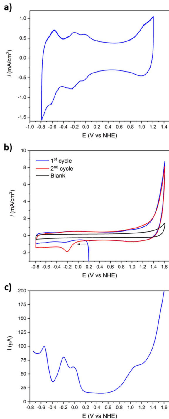
Fig. 3 Electrochemical behavior of \text{Ba}[\text{Co}_2\text{Fe}_2\text{-WS}]/\text{Nafion} ink (a) CV in the -0.8 to +1.2 V potential range. (b) CV, initial scan direction towards cathodic potentials as indicated by the arrow. The presence of \text{O}_2 due to OER catalysis is confirmed by the reduction peak appearing at -0.33 V during the second cycle. Note that the blank measurement shown corresponds to the second cycle in which the \text{O}_2 reduction peak is absent. (c) Differential pulse voltammetry measurement. The experiments were conducted in a single-cell under \text{N}_2 atmosphere at \text{pH} 7.2 , 50 mM \text{KPi} buffer, using \text{KNO}_3 (1 M) as electrolyte. The scan rate for the CV was 100\text{ mV s}^{-1} .
