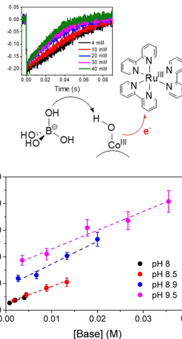
Fig. 5 Representation of photoinduced proton coupled electron transfer occurring at the surface of Co 3 O 4 nanoparticles WOC, where the electron is transferred to Ru III (bpy) 3 3+ and the proton to borate; below is reported the dependence on the rate constant on the pH and on the concentration of the borate base, indicative of a general base catalysis. Reprinted from ref. 77 with permission from the Royal Society of Chemistry, copyright 2018.
