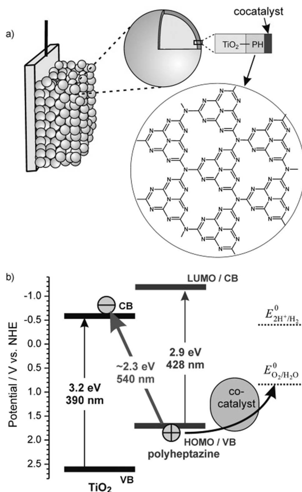
Fig. 27 (a) Hybrid photoelectrodes based on nanocrystalline TiO 2 sensitized with polyheptazine and loaded with a CoO x WOC, and (b) energy levels evidencing the direct optical charge-transfer excitation of an electron from the polyheptazine HOMO into the conduction band of TiO 2 . Reprinted from ref. 134 with permission from Springer, copyright 2013.
