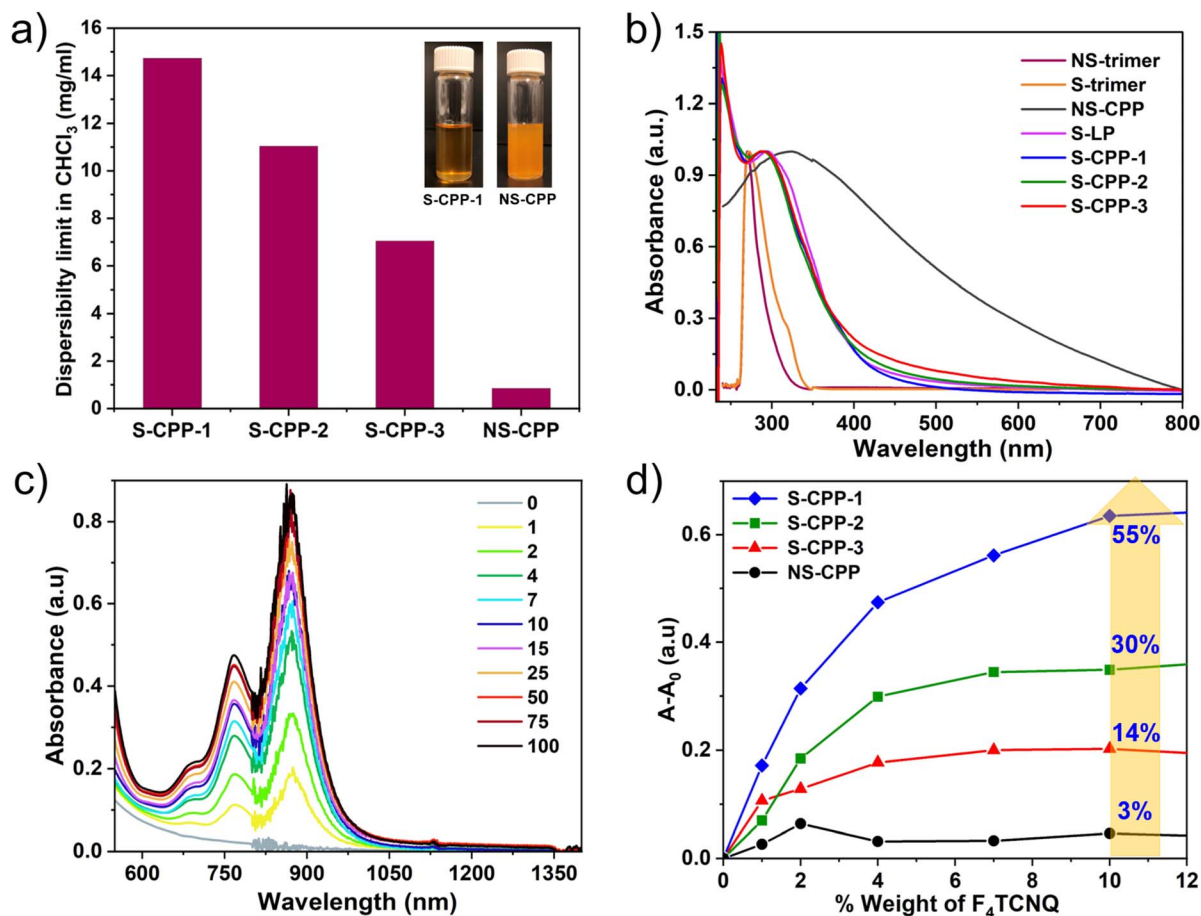
Fig. 4 (a) Dispersibility limit of CPPs in \text{CHCl}_3 ( 1 \text{ mg mL}^{-1} dispersions of S-CPP-1 and NS-CPP are shown for comparison in the inset); (b) UV-vis absorption spectra of CPPs, S-LP, trimers in chloroform; (c) increase in the absorbance of \text{F}_4\text{TCNQ}^- upon increasing the loading of \text{F}_4\text{TCNQ} in S-CPP-1 solution (legend: weight% of \text{F}_4\text{TCNQ} with respect to S-CPP-1); (d) change in absorbance at 873 nm (corresponding to the absorbance of \text{F}_4\text{TCNQ}^- ) as the weight% of \text{F}_4\text{TCNQ} is increased in solution for S-CPP-1–3 and NS-CPP, doping efficiency of CPPs increases as the porous polymer network solvodynamic size decreases.
