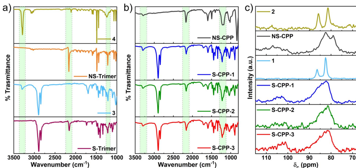
Fig. 2 ATR-IR spectra of (a) arylmonoacetylenes (3 & 4) and trimers; (b) S-CPP-1–3 and NS-CPP (highlighted in green from left to right: ethynyl – C–H stretch, alkyne –C \equiv C– stretch, and –P–C– stretch); (c) ^{13}\text{C} CP-MAS-NMR spectra of monomers (1 & 2) and CPPs are compared to highlight the change in ethynyl carbons chemical shifts and peak widths upon network formation ( \delta : ca. 86.4 and 82.5 ppm for monomer 1 and \delta : ca. 103.5 and 82.1 ppm for S-CPP-1).
