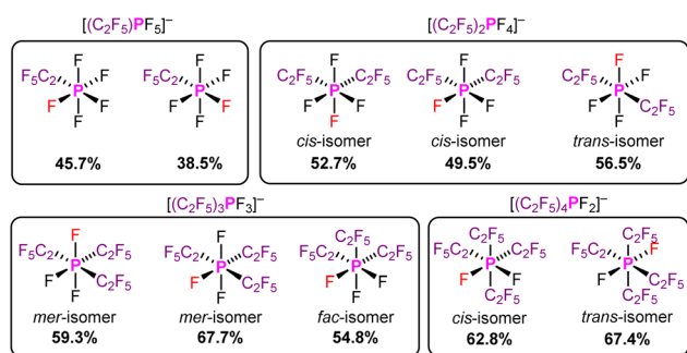
Fig. 5 Pentafluoroethyl(fluoro)phosphoranes (C 2 F 5 ) n PF 5-n and their %V Bur values.
