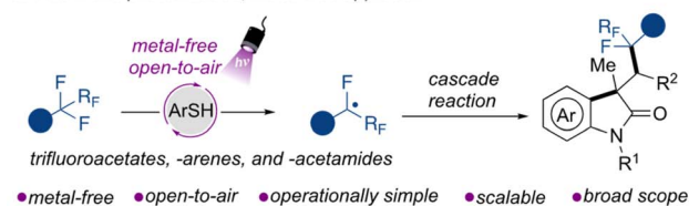
Fig. 1 Previous approaches to preparing difluoroalkylated compounds.
